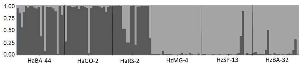
Figure 3. Bar plot for K = 2 clusters for Helicoverpa armigera (HaBA-44, HaGO-2, and HaRS-2) and H. zea (HzMG-4, HzSP-13, and HzBA-32) individuals assigned by STRUCTURE, based on seven microsatellite loci. Each color (dark and light gray) represents a different cluster.
