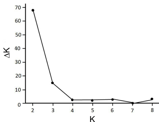
Figure 2. Graphical plot of \Delta K for Helicoverpa armigera and H. zea ; the maximum value of \Delta K was considered to be the value of K (genetic groups or clusters) that best fit the data; K = 2 .
